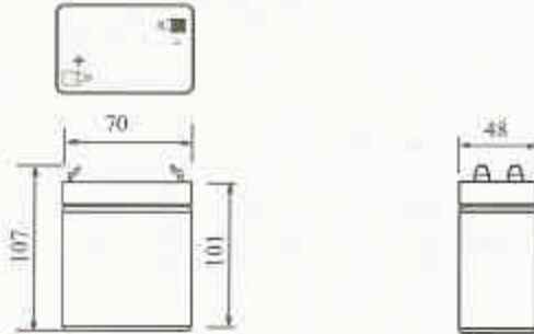
Dimensions of Standard Cover with F1 terminal (Fasten Tab No 187E) (mm)
