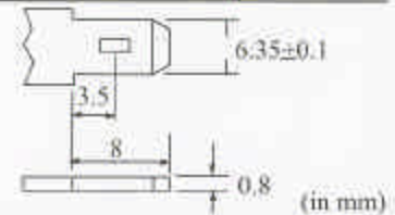
Optional Terminal F2 (Fasten Tab No.250E)
