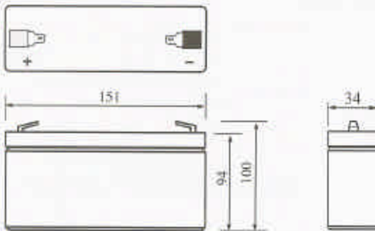
Dimensions (mm)
